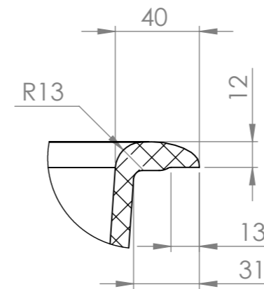
DETAIL B SCALE 2 : 5
