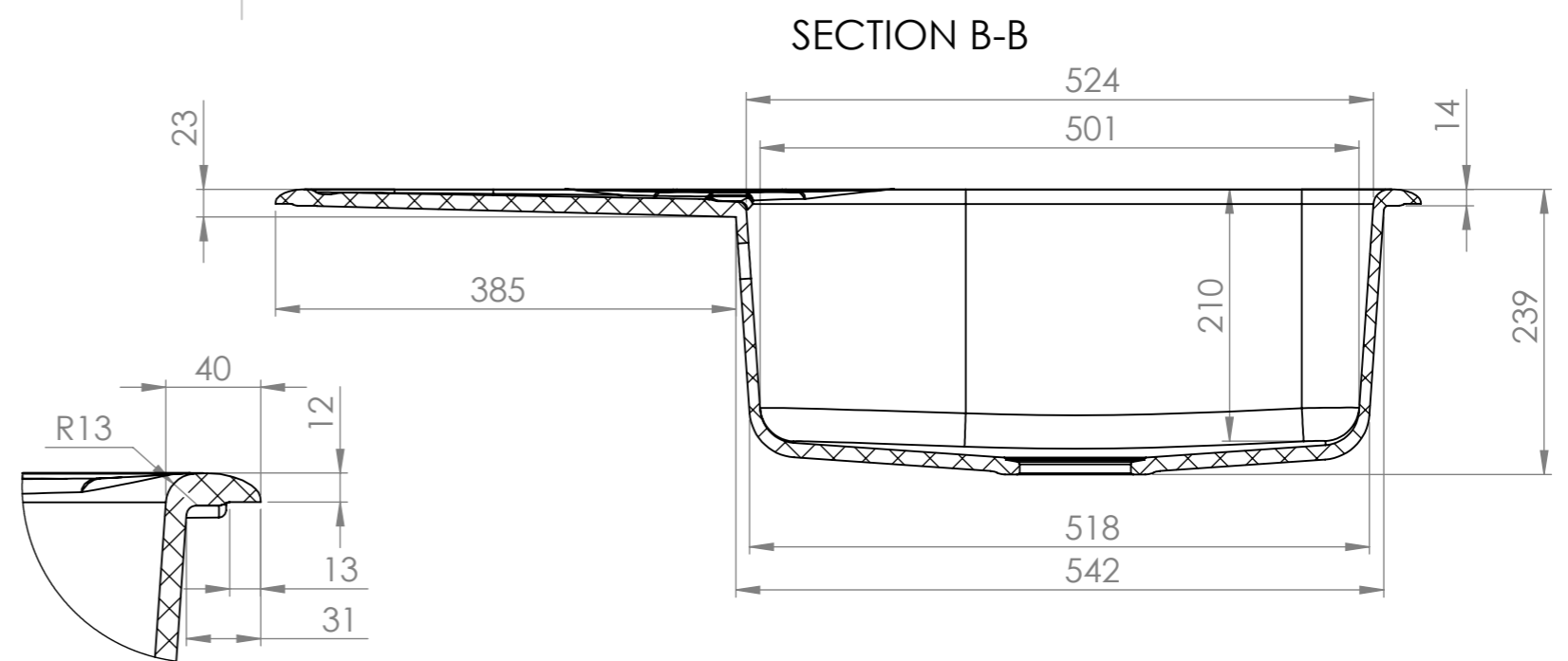
DETAIL C SCALE 1 : 3
