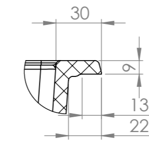
DETAIL C SCALE 2 : 5
