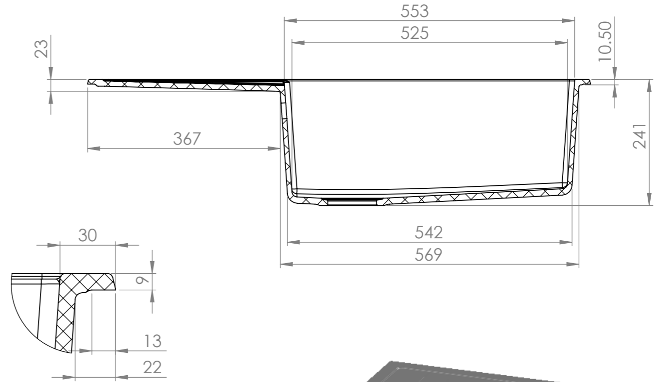
DETAIL C SCALE 1 : 2
